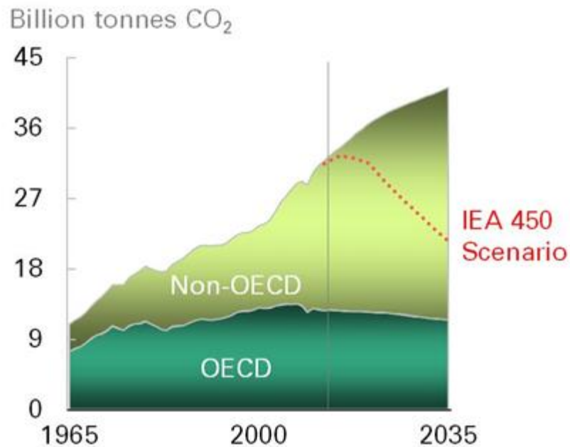
Emissions by region
